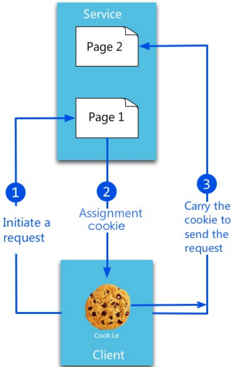
Figure 6.1 cookie principle.
