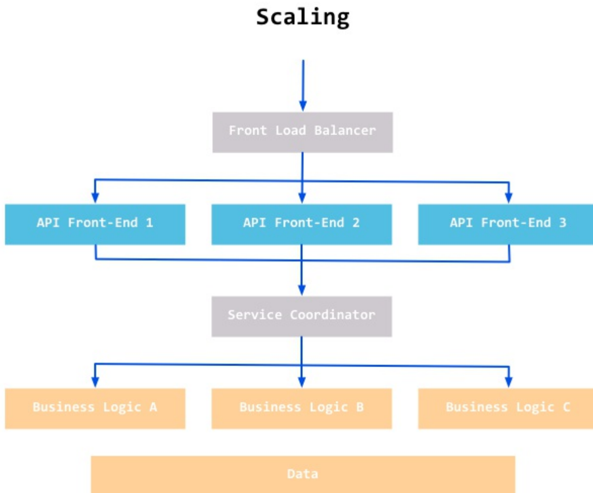
Figure 8.6 REST's expansibility.
