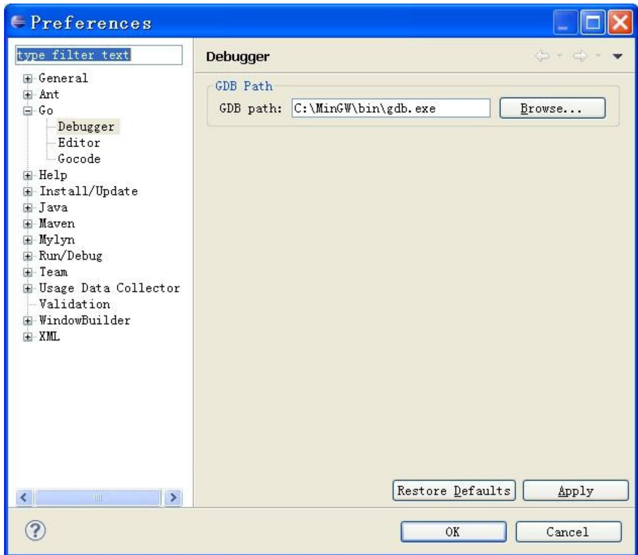
Figure 1.14 gdb Setting
