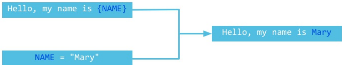
Figure 7.1 Template mechanism
