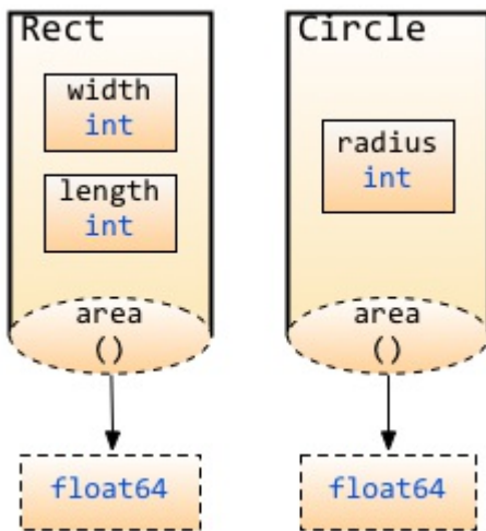
Figure 2.9 Methods are different in different structs
