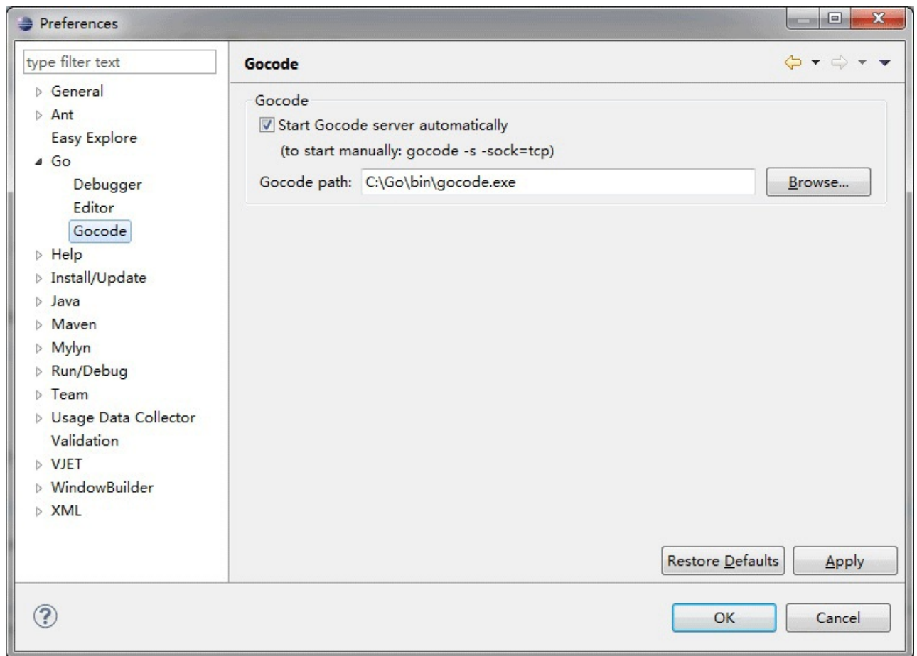
Figure 1.13 gocode Setting
