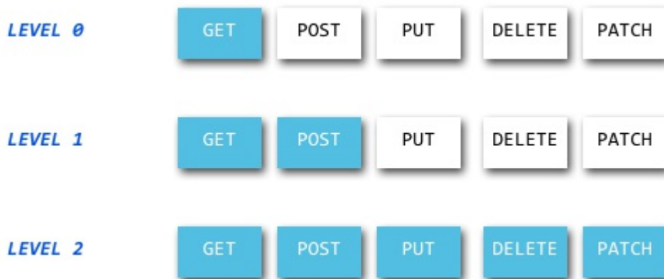
Figure 8.7 REST's level.
