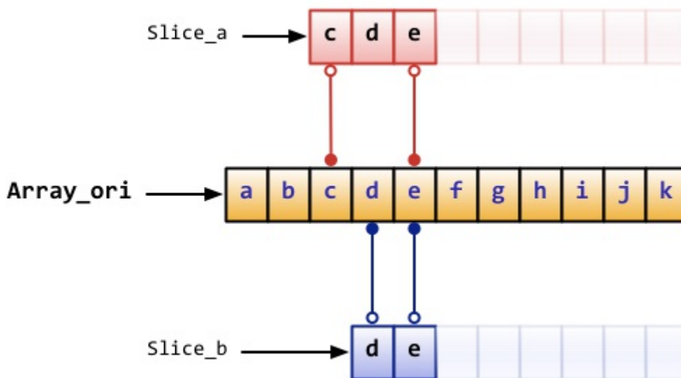
Figure 2.3 Correspondence between slice and array
