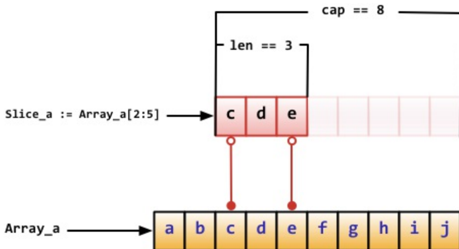
Figure 2.4 Array information of slice
