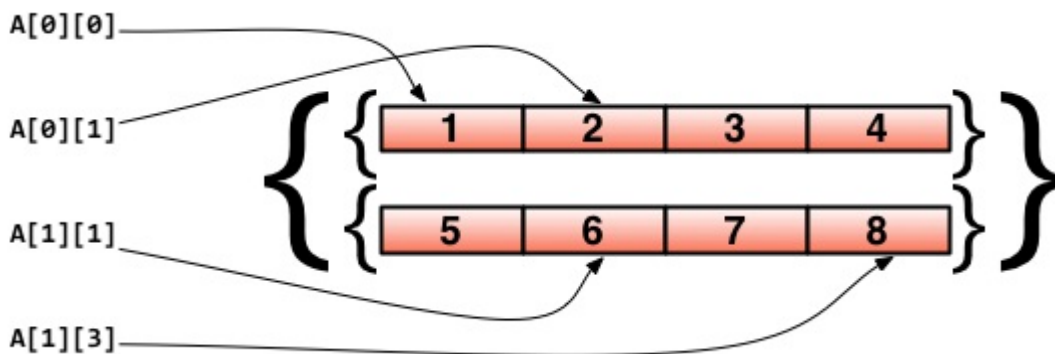
Figure 2.2 Multidimensional array mapping relationship
