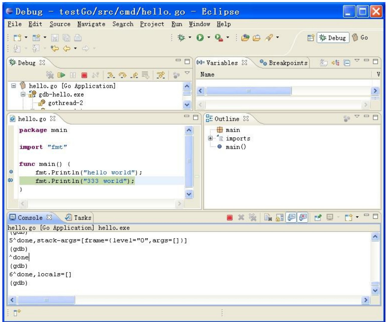
Figure 1.16 Test Go program in Eclipse
