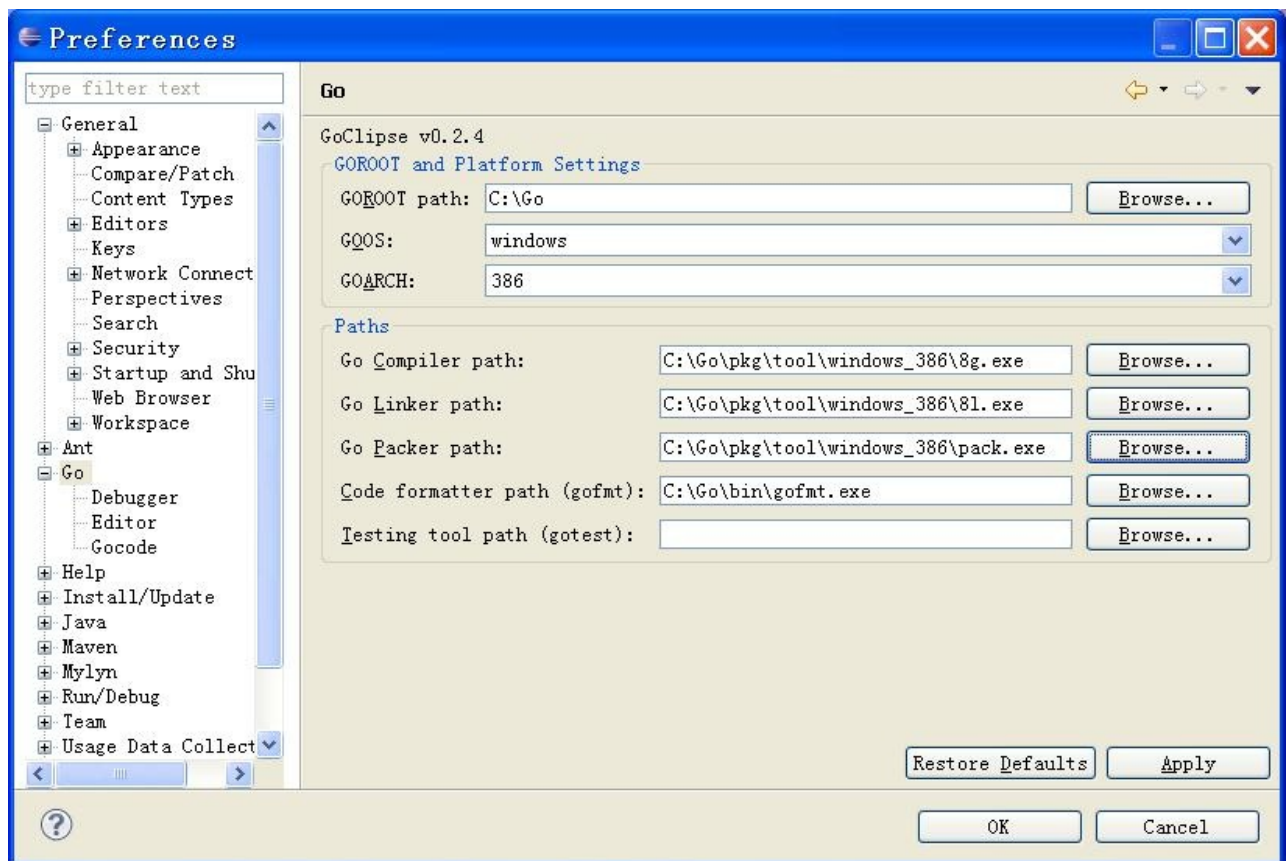
Figure 1.12 Go Setting in Eclipse
