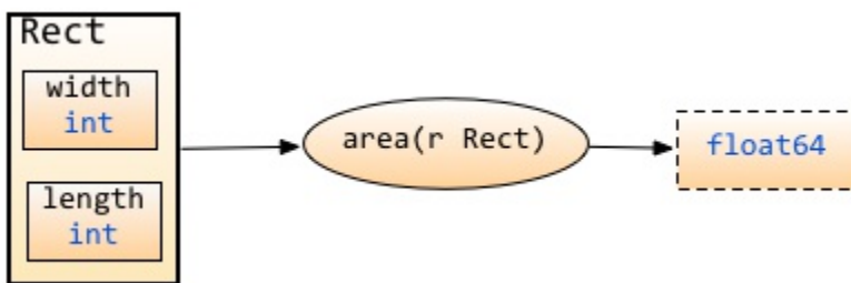
Figure 2.8 Relationship between function and struct
