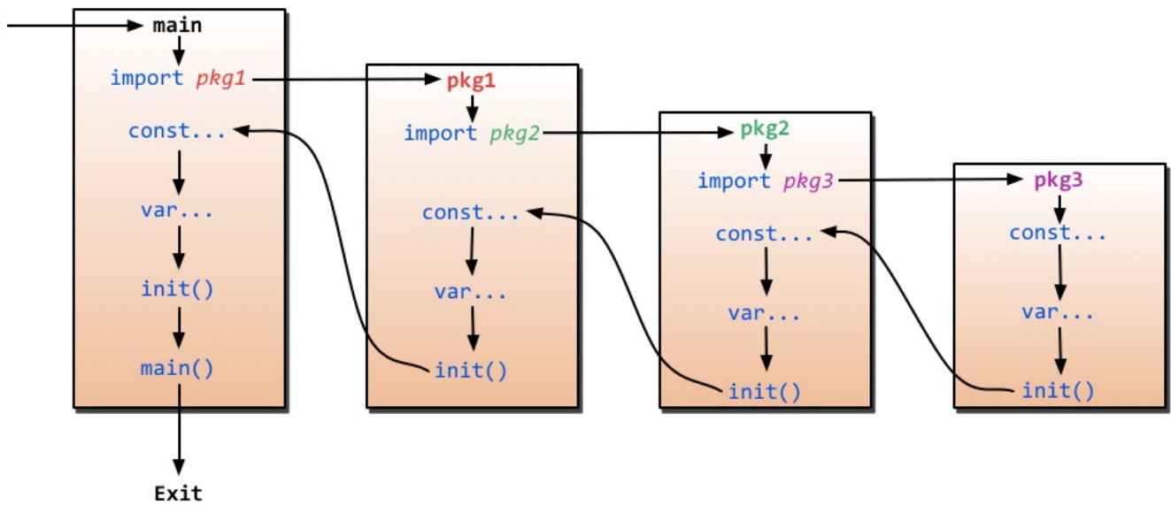
Figure 2.6 Flow of programs initialization in Go
